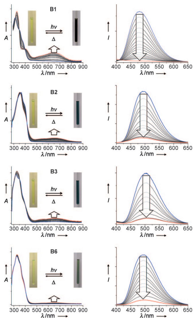
Figure 2. Changes in the absorption (left) and emission (right) spectra of B1 , B2 , B3 , and B6 in toluene upon irradiation at 365 nm. Inset: Photographs showing the color of the compounds before and after irradiation.
