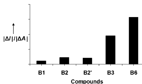
Figure 4. The plot of the ratio of total emission intensity change |\Delta I| versus the total absorption changes |\Delta A| for the monoboryl and polyboryl compounds.
